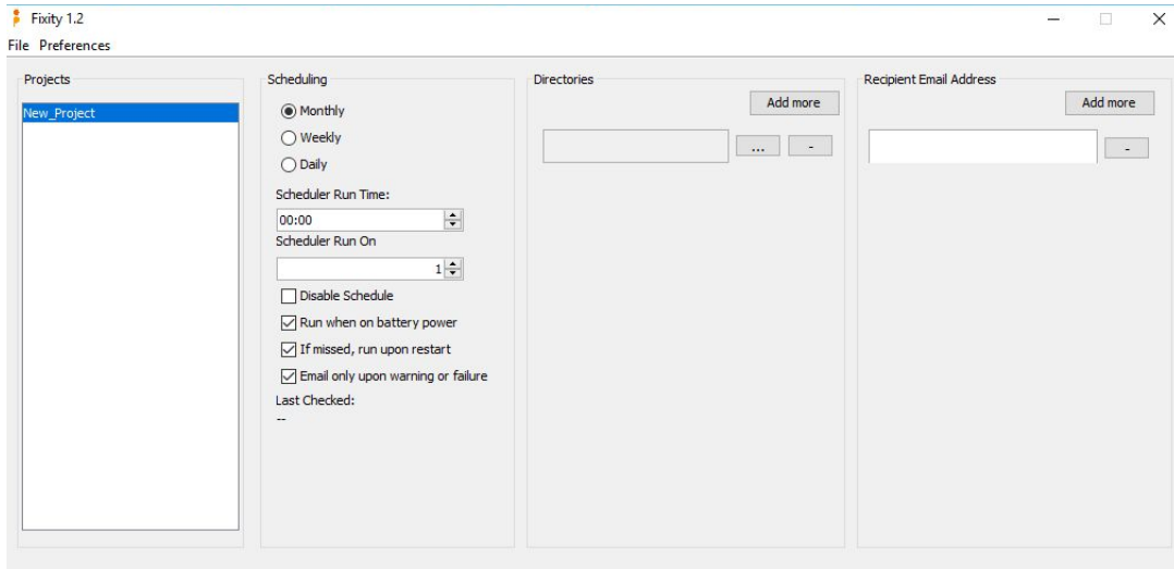
Figure 8: Screenshot of Fixity version 1.2 interface for Windows. Note that all options will appear greyed out until you create a project.
