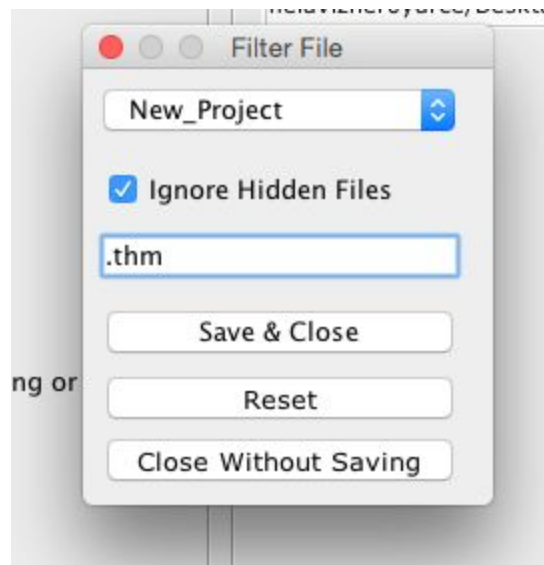
Figure 12: Fixity Filter File detail with “Ignore Hidden Files” selected and sample file format pattern to block.
